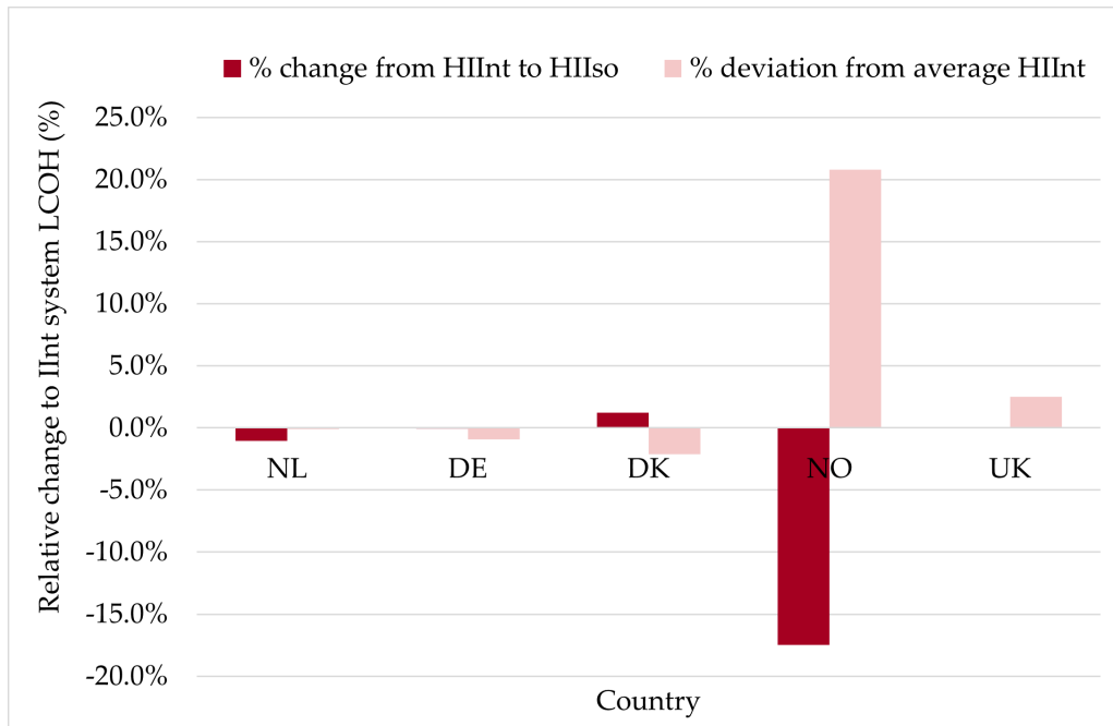
Figure 25: Hydrogen networks cost changes per country. In red (left columns), the % change in LCOH from an interconnected network (HIInt) to an isolated network (HIIso). In pink (right columns), the % deviation in LCOH from the average LCOH of the interconnected (HIInt) scenario.
