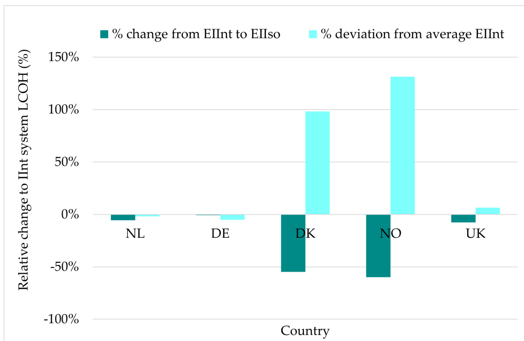
Figure 26: Electricity grids costs changes per country. In green (left columns), the % change in LCOH from an interconnected grid (EIInt) to an isolated grid (EIIso). In blue (right columns), the % deviation in LCOH from the average LCOH of the interconnected (EIInt) scenario.
