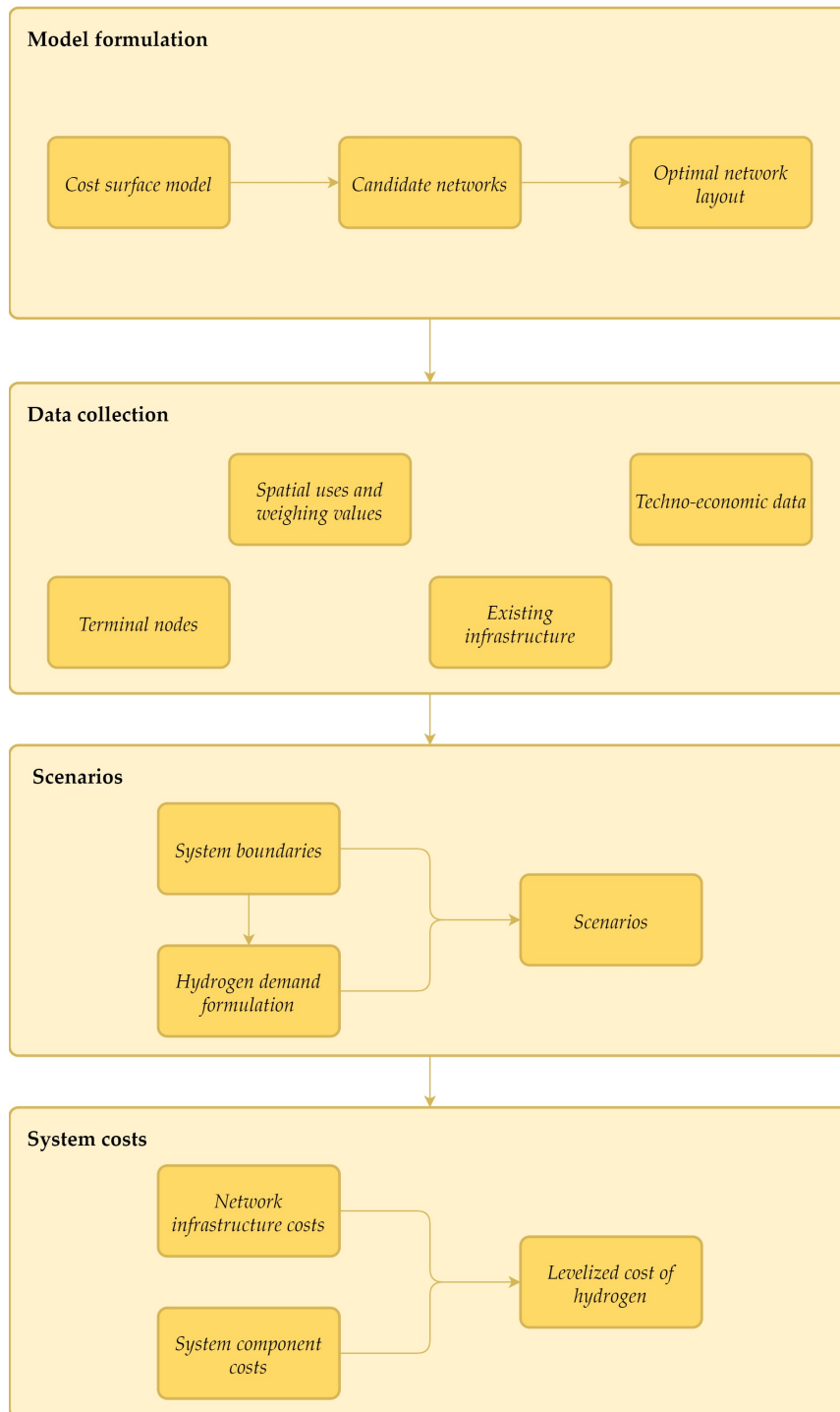
Figure 8: Methodology flowchart.
