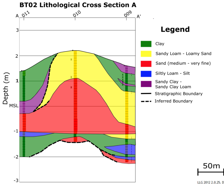
Figure 17 Cross section 1 depicting subsurface interpretation of architecture, sediment types and boundaries, created using the LLG software
