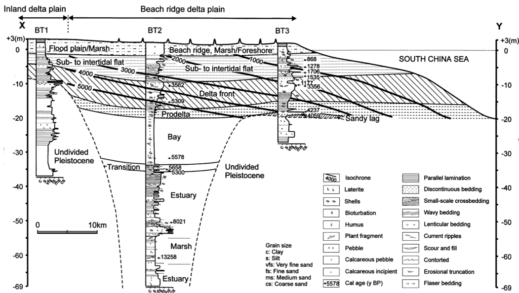
Figure 8 Cross section and core logs of sedimentary facies in the lower Mekong Delta plain in the province of Ben Tre from (Ta et al., 2002a)
