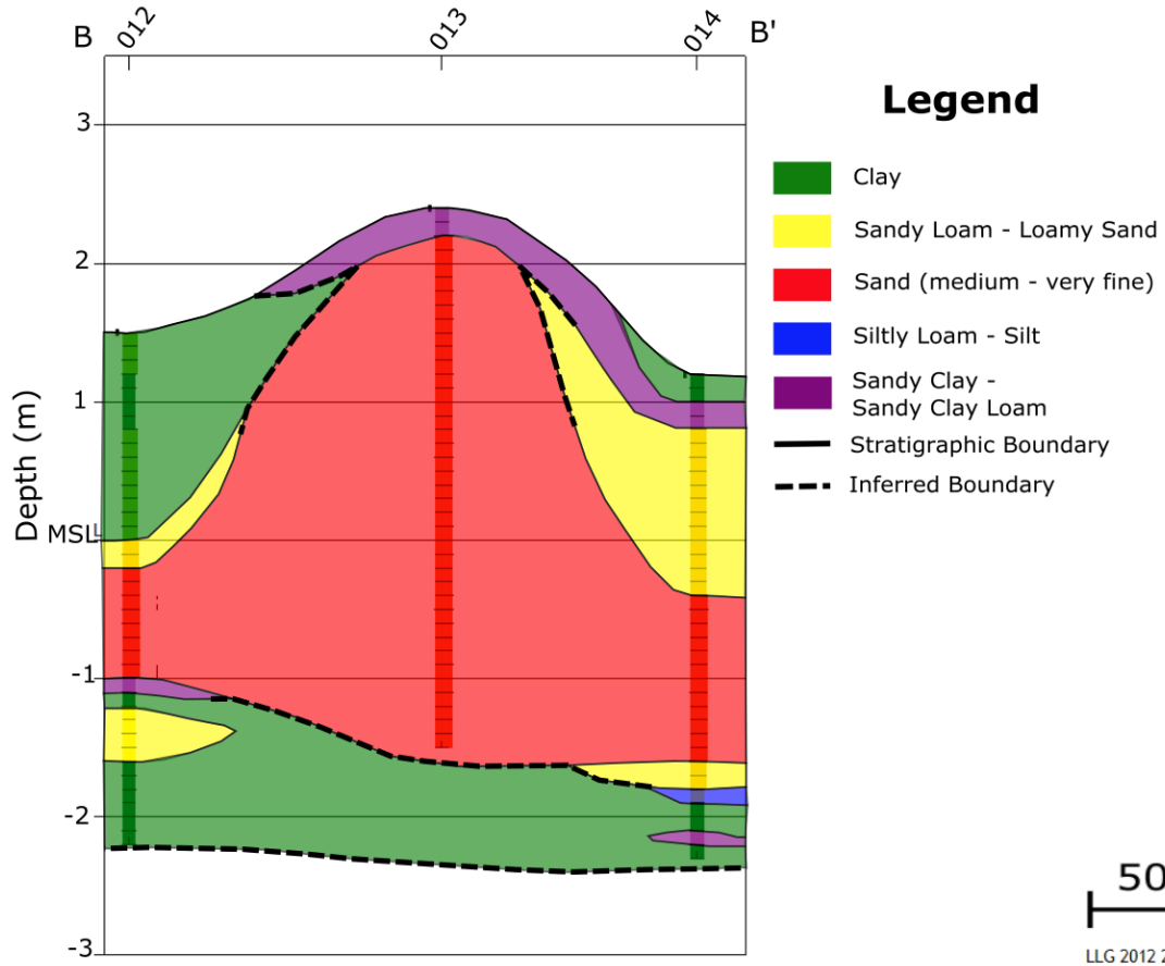
Figure 18 Cross section 2 depicting subsurface interpretation of architecture, sediment types and boundaries, created using the LLG software.
