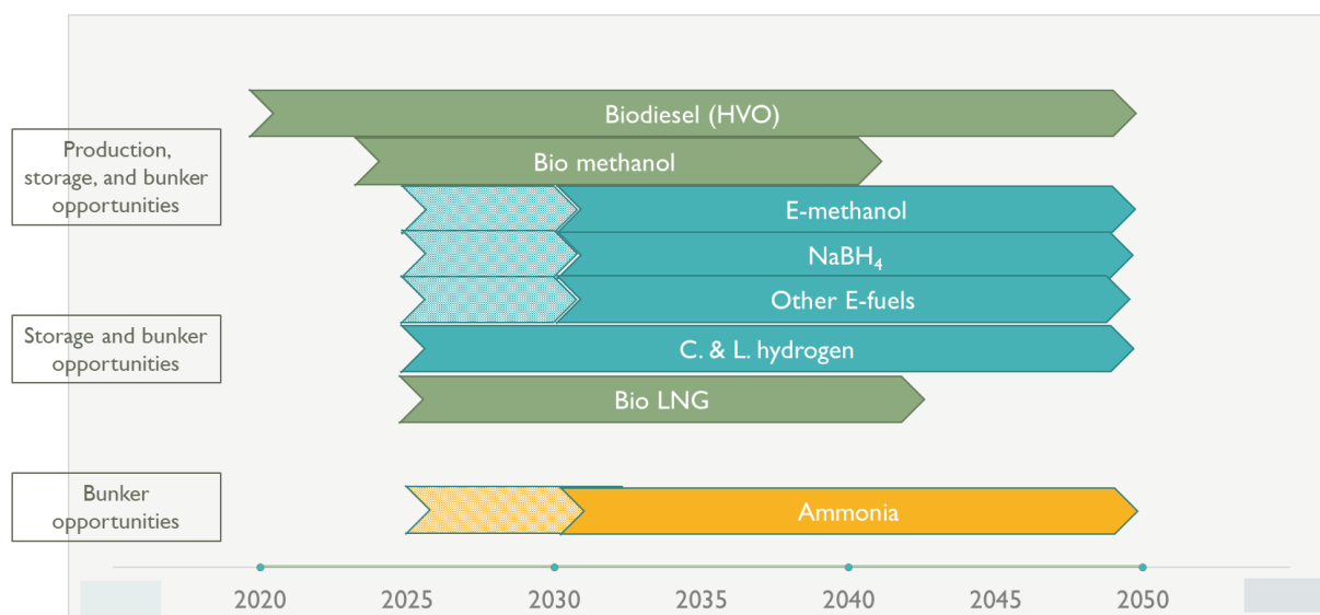
Figure 21: Attractive alternative fuels for coastal and inland vessels according to added value Amsterdam port
