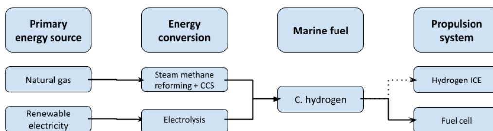
Figure 9: Production pathways compressed hydrogen (dotted pathways are not preferred)
