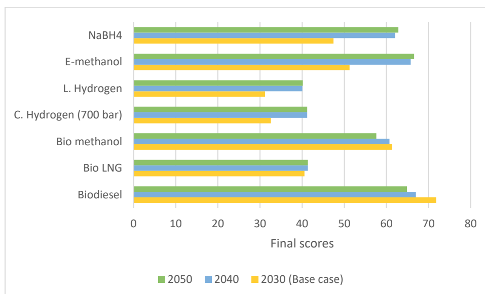
Figure 15: Sensitivity analysis - Long-term scenario
