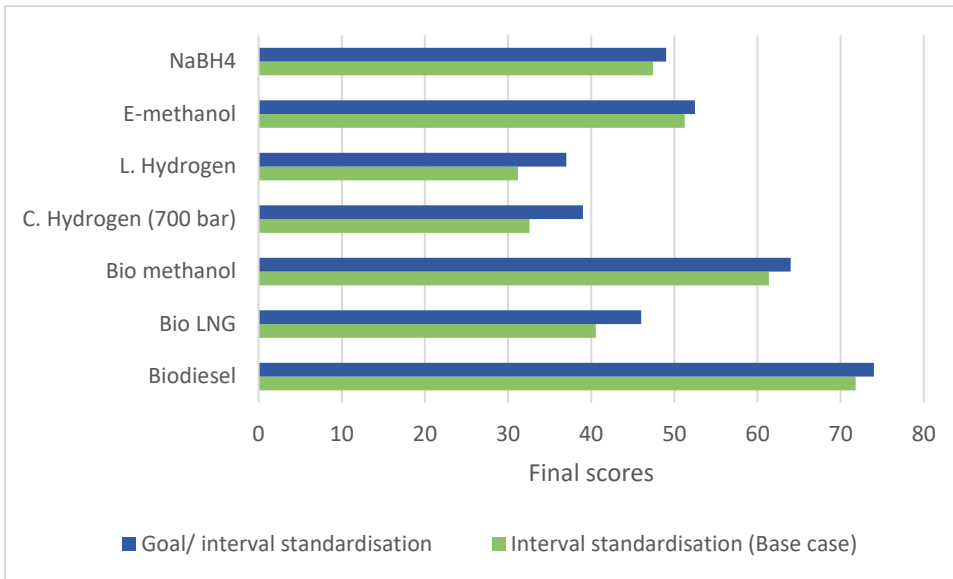
Figure 19: Sensitivity analysis - Different standardisation method
