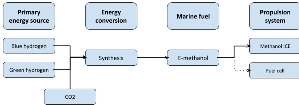
Figure 11: Production pathways e-methanol (dotted pathways are not preferred)
