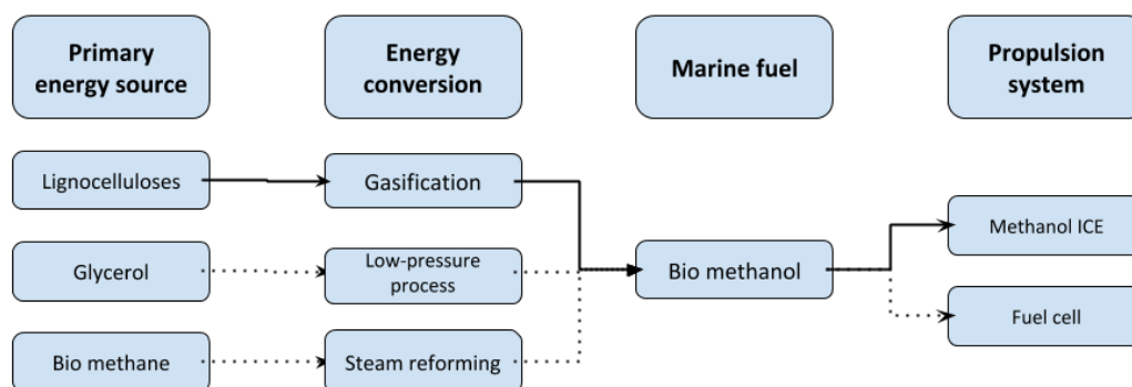
Figure 8: Production pathways bio methanol (dotted pathways are not preferred)
