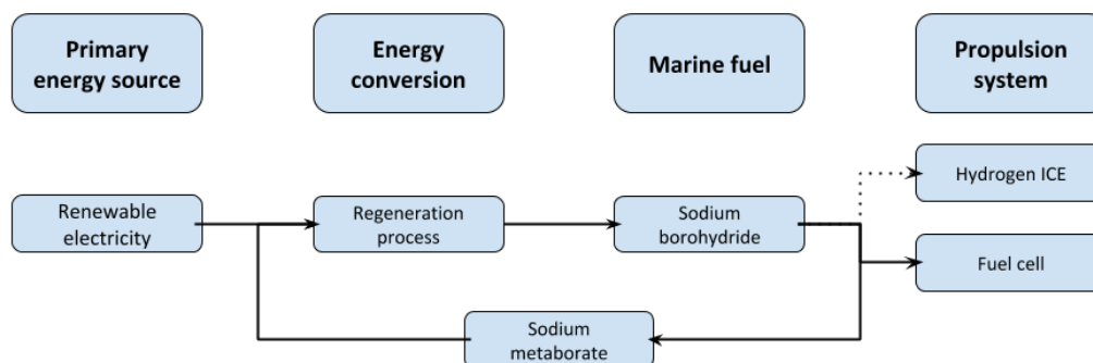
Figure 12: Production pathways sodium borohydride (dotted pathways are not preferred)
