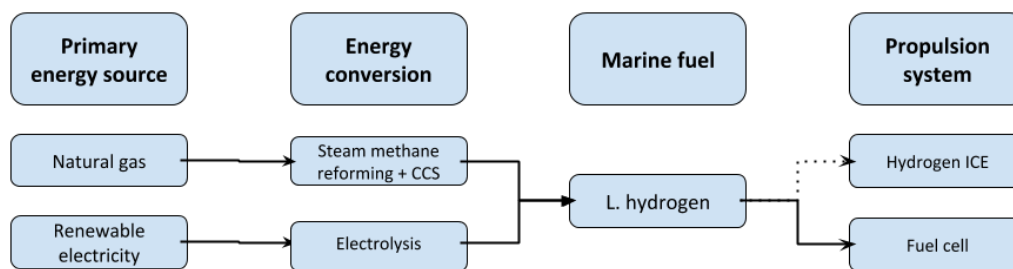
Figure 10: Production pathways liquid hydrogen (dotted pathways are not preferred)
