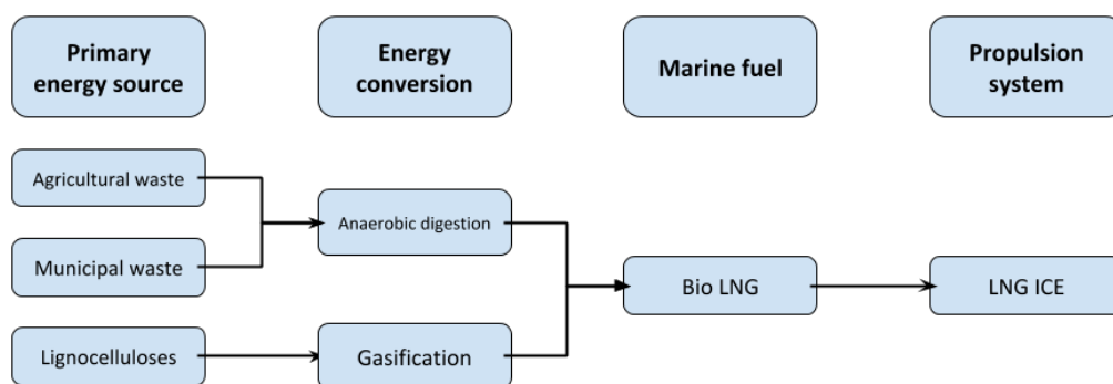
Figure 7: Production pathways bio LNG (dotted pathways are not preferred)
