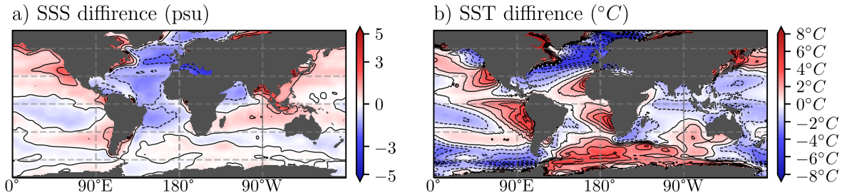
Figure 4: Errors in surface forcing. As a difference between ECMWF-1° forcings and their zonal mean. Here positive values are over estimations of the forcings. Errors for: a) the SSS difference with contours every 1 psu and b) the SST difference with contours every 1 °C
