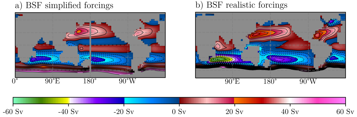
Figure 15: Barotropic stream function with contours every 5 Sv. For a) the simplified forcings based on the ECMWF-1° as explained in section 2.2.2 and b) realistic ECMWF-4° forcings (ECMWF 2015)
