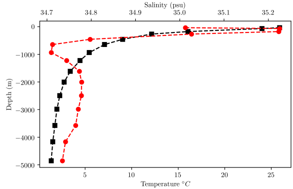
Figure 3: Temperature and salinity profiles at 2°N. Black squares indicate the Temperature (°C) profile and red circles indicate the salinity (psu) profile. Profiles from ECMWF 2020 scaled to 15 depth layers with grid stretching.
