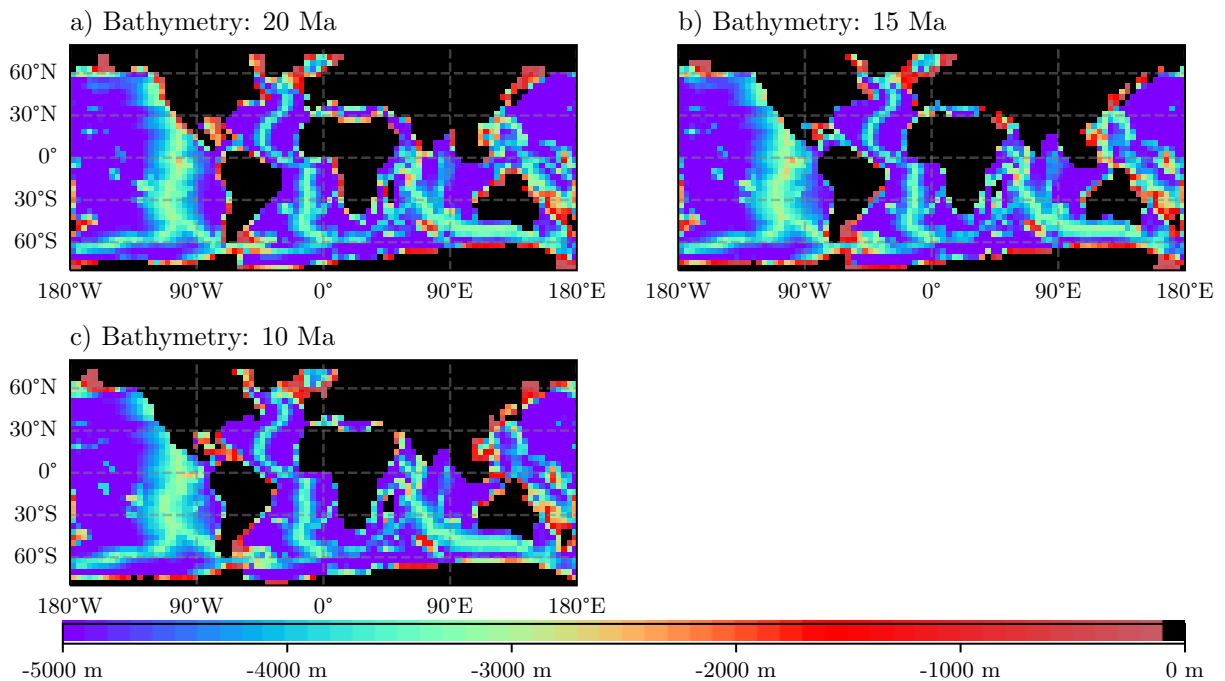
Figure 12: Miocene bathymetries, black squares show the land mask used. The bathymetries for (a) 20 Ma. (b) 15 Ma Here, the closure of the Thetys Seaway is seen which connects the African continent to the Eurasian continent and stops the northern flow of water between the Indian and Atlantic Oceans. (c) 10 Ma Here the panama seaway is seen to become much more shallow. Also the Indonesian passage has shrunk drastically in this period.
