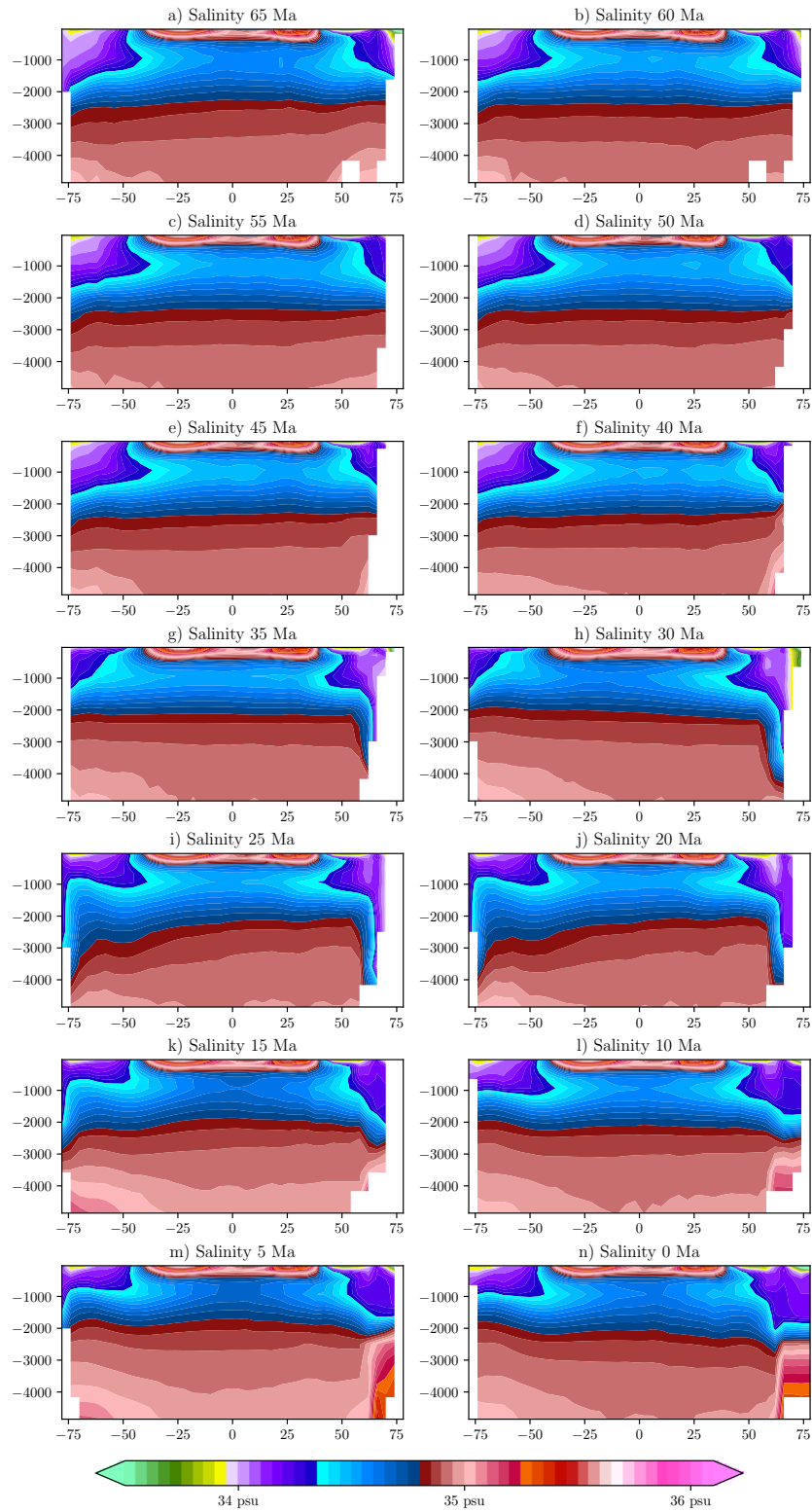
Figure 29: Latitude depth profile of the zonal mean Salinity
