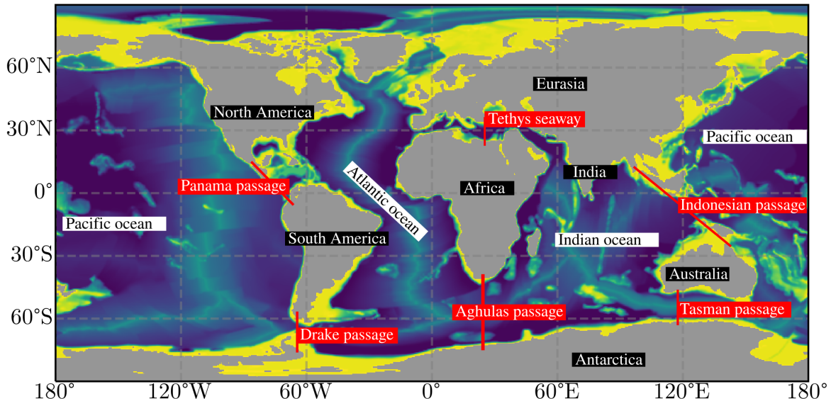
Figure 8: Schematic image showing the 30 Ma bathymetry in 0.5^\circ \times 0.5^\circ . Overlaid in red are the passages we study. In black the continents and in white the oceanic basins.
