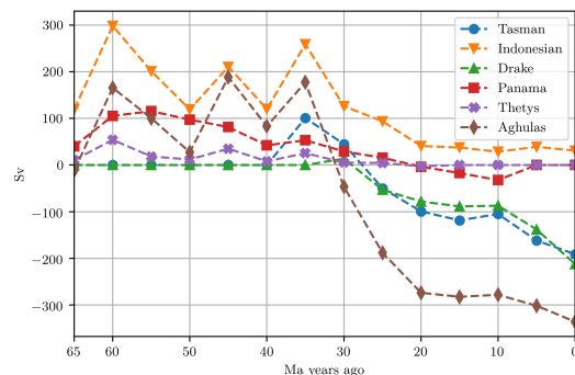
Figure 17: Total volume transport in Sverdup ( 10^6 m^3 s^{-1} ) running from 65 million years ago to the present day situation. Positive values indicate transport to the west. Passage names as defined in fig. 7.
