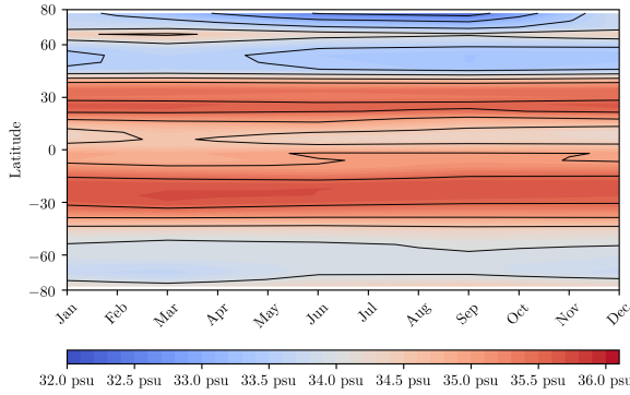
(c) SSS profile ( psu )
