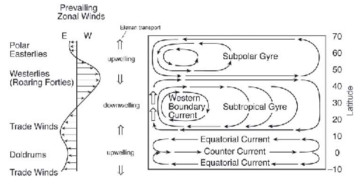
Figure 6: Schematic of the barotropic stream function based on the Sverdrup relation. Showing the subpolar and subtropical Gyres and equatorial currents. Figure taken from John Marshall 2012
