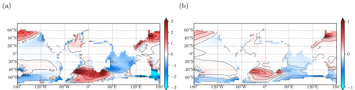
Figure 25: Comparison between late Eocene (35Ma) and early Miocene (20Ma) for: a) Temperature ( ^{\circ}C ) differences (positive values indicate warming) and b) Salinity ( psu ) differences (positive values indicate higher salinity)
