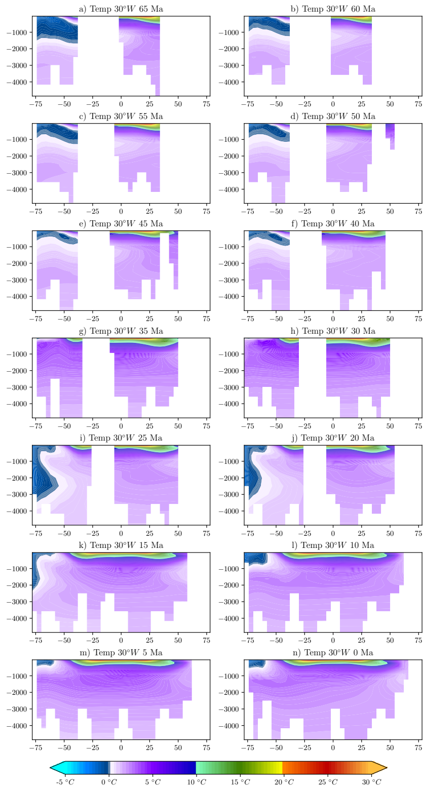
Figure 28: Latitude depth profile of the Temperature in the Atlantic (178°W)
