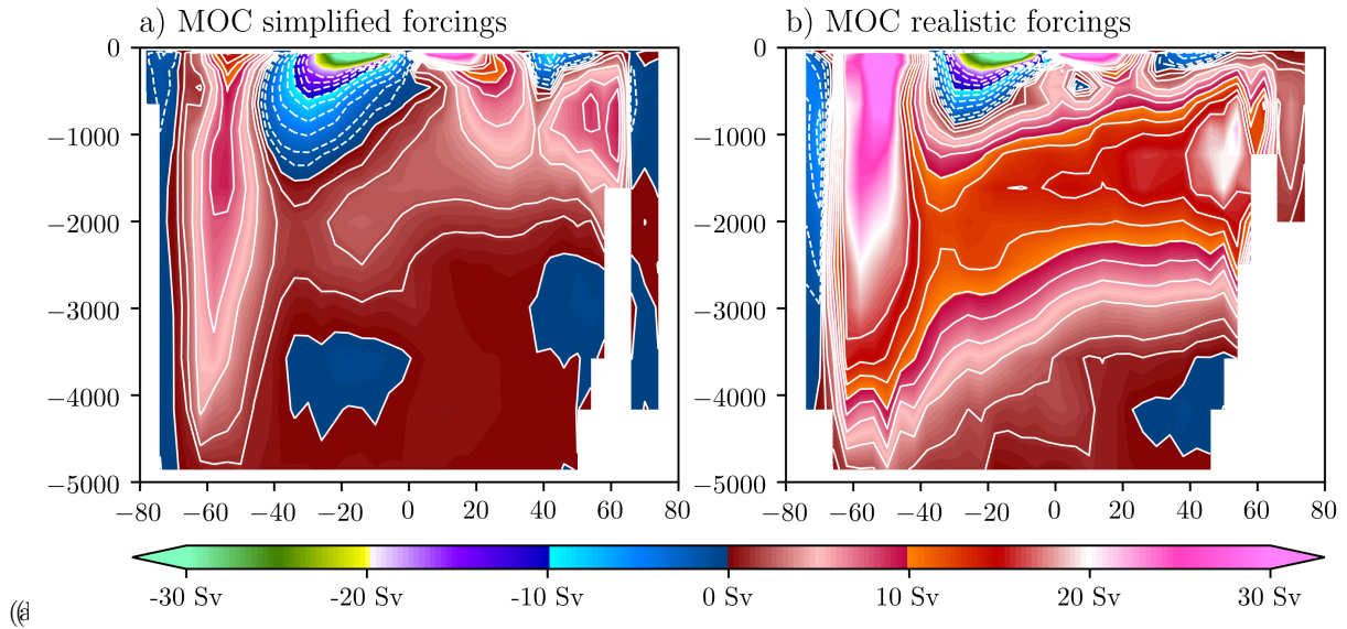
Figure 16: MOC stream function with contours every 2 Sv. For a) the simplified forcings based on the ECMWF-1° as explained in section 2.2.2 b) realistic ECMWF-4° forcings (ECMWF 2015). Negative values (dashed lines) indicate counterclockwise circulation. Here a large difference between the forcings is clearly visible
