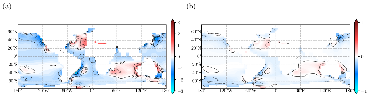
Figure 26: Comparison between early Miocene (20Ma) and late Miocene (10Ma) for: a) Temperature ( ^{\circ}C ) differences (positive values indicate warming) and b) Salinity ( psu ) differences (positive values indicate higher salinity)
