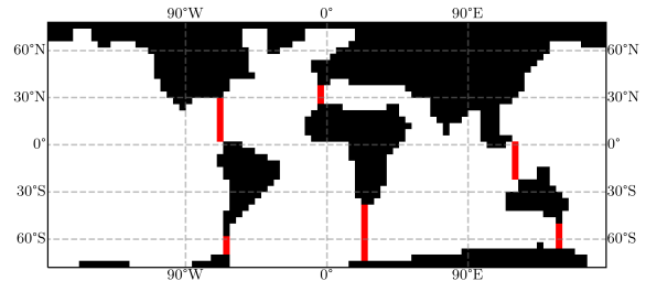
Figure 7: Example of the chosen grid cells for individual passages for 20Ma. The land mask shown here is the land mask excluding grid cells used for the BSF boundary conditions and is thus not the same as the land mask used for the model itself.
