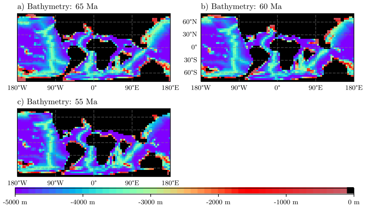
Figure 9: Paleocene bathymetries, black squares show the land mask used. The bathymetries for (a) 65 Ma including the Kohistan-Ladakh Arc (b) 60 Ma showing submergal of the Kohistan-Ladakh Arc (c) 55Ma here the gap between africa and south America is seen to grow.
