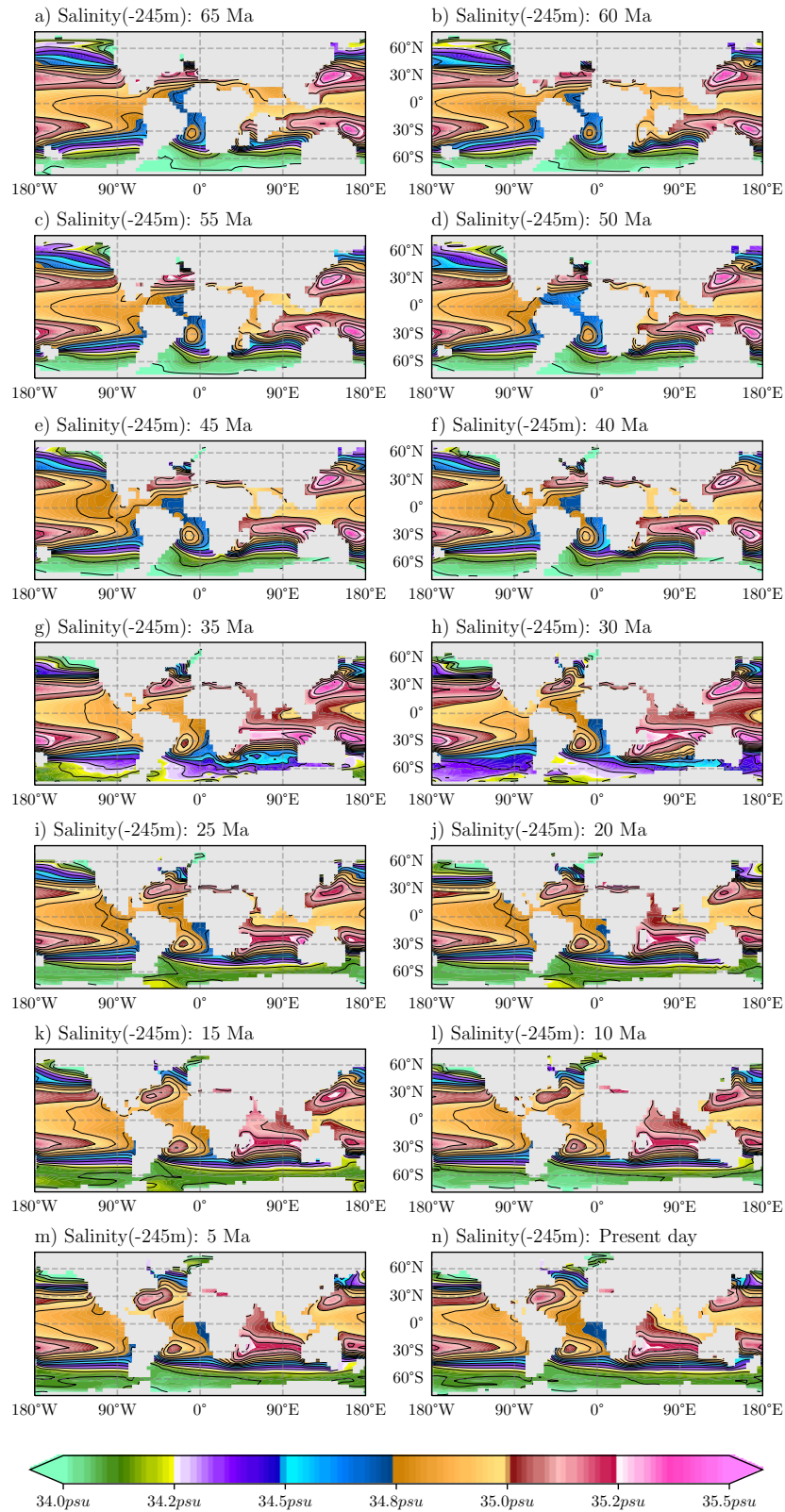
Figure 22: Salinity at 245m depth for each time step. Contours every 0.1psu Here the Eocene-Oligocene boundary is seen as one of the major changes along with fluctuations in the Indian ocean.
