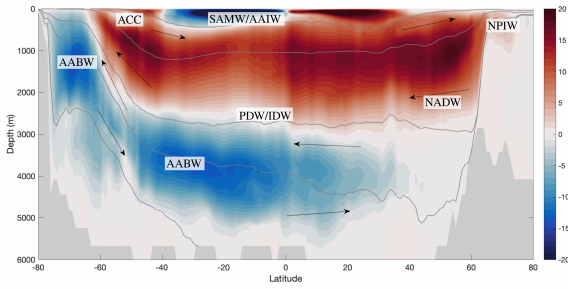
Figure 5: Meridional overturning circulation from observations taken from Forget et al. 2015. With schematic arrows indicating flow direction. Also including locations of major overturning flows. AABW: Antarctic Bottom Water, NADW: North Atlantic Deep Water, NPIW: North Pacific Intermediate Water, SAMW: Subantarctic Mode Water, AAIW: Antarctic intermediate Water, ACC Antarctic Circumpolar Current.
