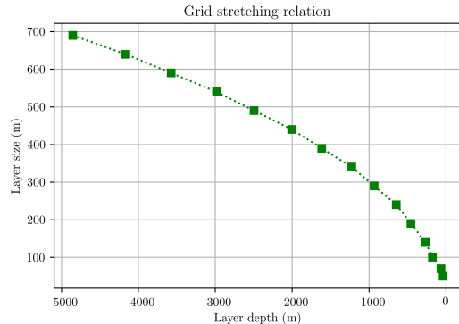
Figure 1: Grid stretching relation used for the model setup. Showing the size of the layer for each layer. Upper layers are shallower than deep water layers.
