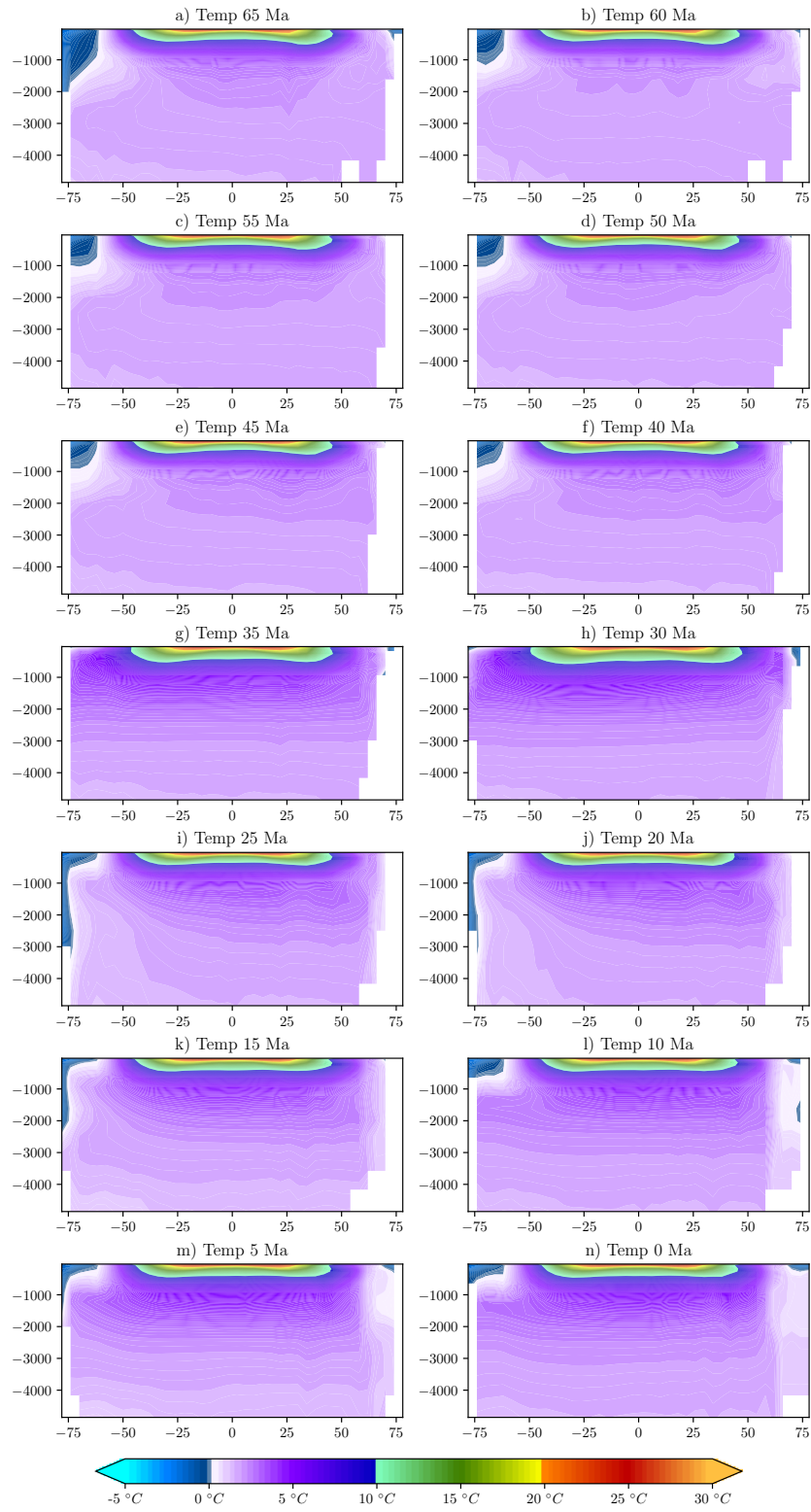
Figure 30: Latitude depth profile of the zonal mean temperature
