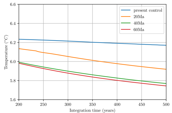
Figure 14: Total globally averaged temperature ( ^{\circ}C ) for Present day (blue), 20Ma (orange), 40Ma (green) and 60Ma (red). From 200 to 500 years of integration. A drift is still observed after 500 years of integration but the models do all appear to converge.
