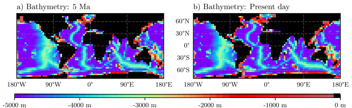
Figure 13: Pliocene bathymetries, black squares show the land mask used. The bathymetries for (a) 5 Ma where the panama passage is closed linking the north and south American continents. (b) The present day situation.
