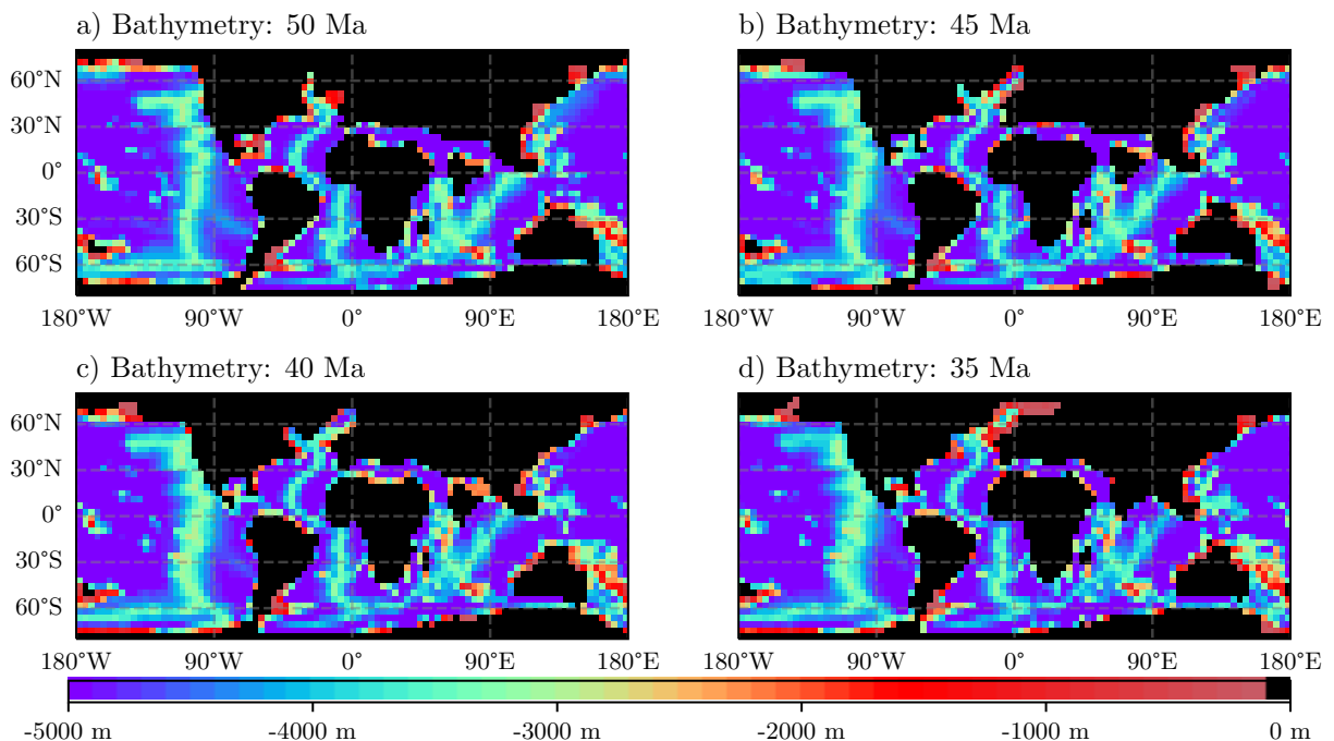
Figure 10: Eocene bathymetries, black squares show the land mask used. The bathymetries for (a) 50 Ma. (b) 45 Ma. (c) 40 Ma. (d) 35 Ma showing the opening of the Tasman passage by the detachment of the Australian continent from Antarctica. Also, water passage over India is closed.
