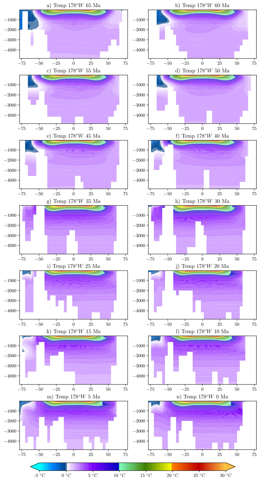
Figure 27: Latitude depth profile of the Temperature in the Pacific (178°W)
