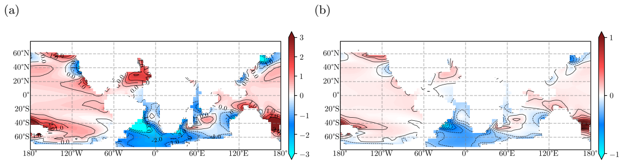
Figure 24: Comparison between late Paleocene (55Ma) and late Eocene (35Ma) for: a) Temperature ( ^{\circ}C ) differences (positive values indicate warming) and b) Salinity ( psu ) differences (positive values indicate higher salinity)
