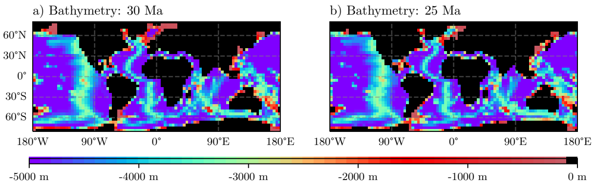
Figure 11: Oligocene bathymetries, black squares show the land mask used. The bathymetries for (a) 30 Ma here the Drake passage is opened, this detaches south America from Antarctica and allows the onset of the ACC (b) 25 Ma where the Thetys Seaway is seen to be slowly shrinking.
