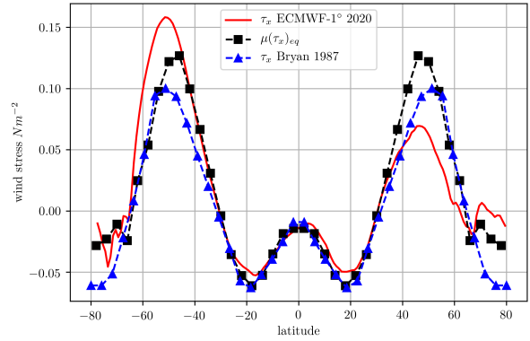
Figure 2: Zonal mean annual forcing profiles for a) The net monthly surface heat flux forcing profile for each latitude. Showing large annual variation in surface heat flux. b) The monthly Sea Surface Temperature (SST) forcing profile. Showing annual variation in the net surface temperature. c) Sea Surface Salinity (SSS) forcing profile showing little annual variation. d) The zonal wind stress profiles ( \tau_x ) that were looked at. The red line shows the zonal average of the ECMWF – 1° forcings. The black squares show zonally averaged ECMWF – 4° forcings that were mirrored along the equator. The Blue triangles show analytic forcing profile from Bryan 1987
