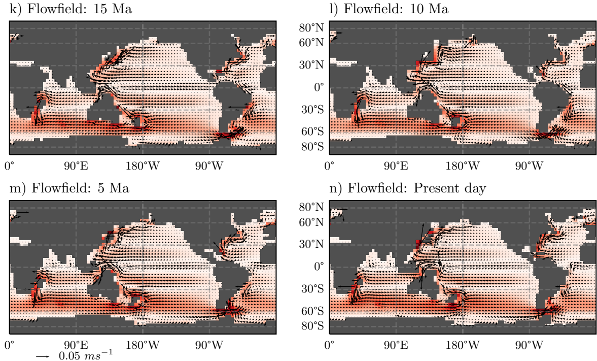
Figure 18: Flow field for each time step as a weighted mean showing the average velocity of each vertical water column in ms^{-1} . Serves to indicate flow direction and relative strength in the oceanic basins. Also serves as a basis to compare results with the shallow water model in Omta and Dijkstra 2003
