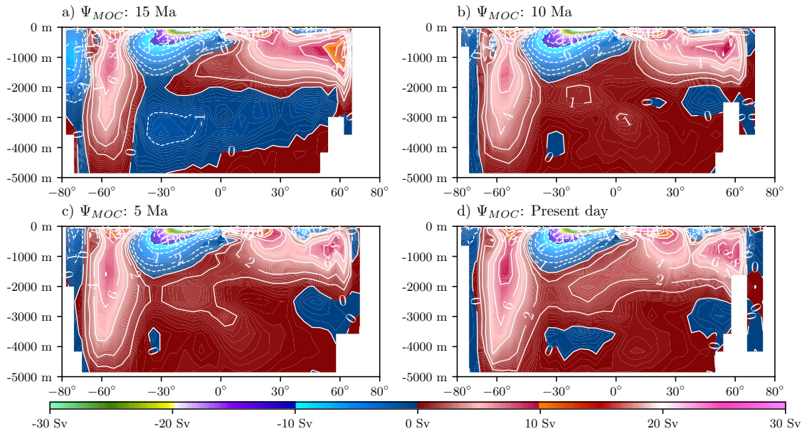
Figure 21: Meridional overturning circulation stream function with contours every 2 Sv and an extra contour for -1\text{Sv} and 1\text{Sv} . Dotted contours indicate negative values. The Deacon cell appearing with the onset of the ACC is particularly visible here.
