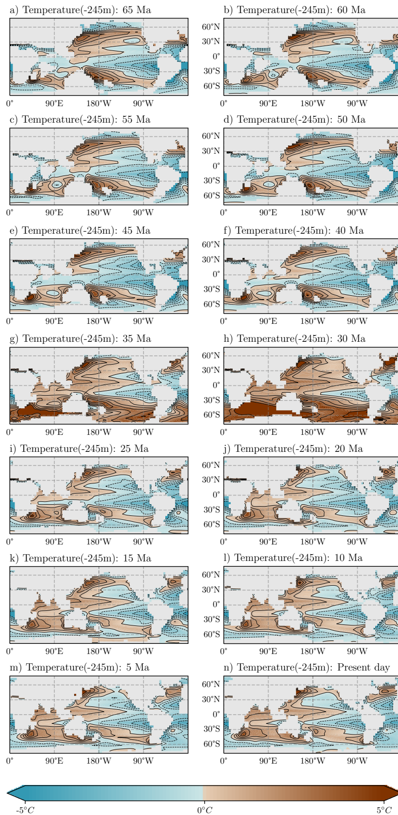
Figure 23: Difference in temperature between initial condition and model output at 245m depth for each time step. Contours every 0.5 °C, here the Eocene-Oligocene boundary is much warmer than the other bathymetries. Also, all of the major ocean gyres are visible.
