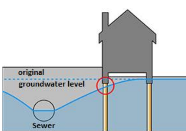
Figure 5.2.4: Lowered groundwater levels exposing wooden pile to oxygen causing pole rot. Source: (Paalrot.info, 2019)
