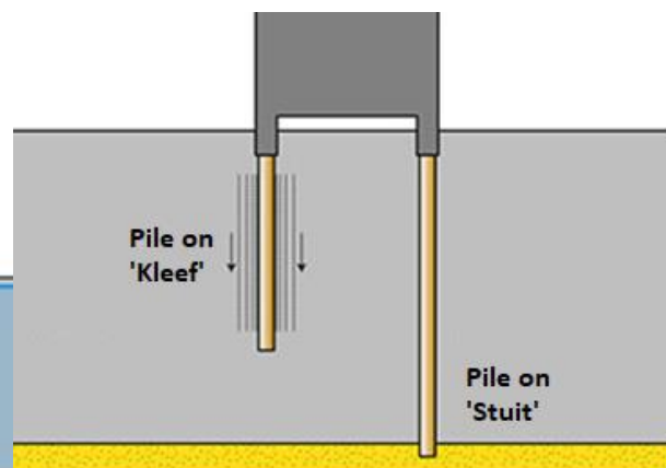
Figure 5.2.5: Negative adhesion "kleef" pulls the foundation pile below resulting in foundation damages. Stuit: when the foundation pile is resting on stable sand layers. Source: (Paalrot.info, 2019)
