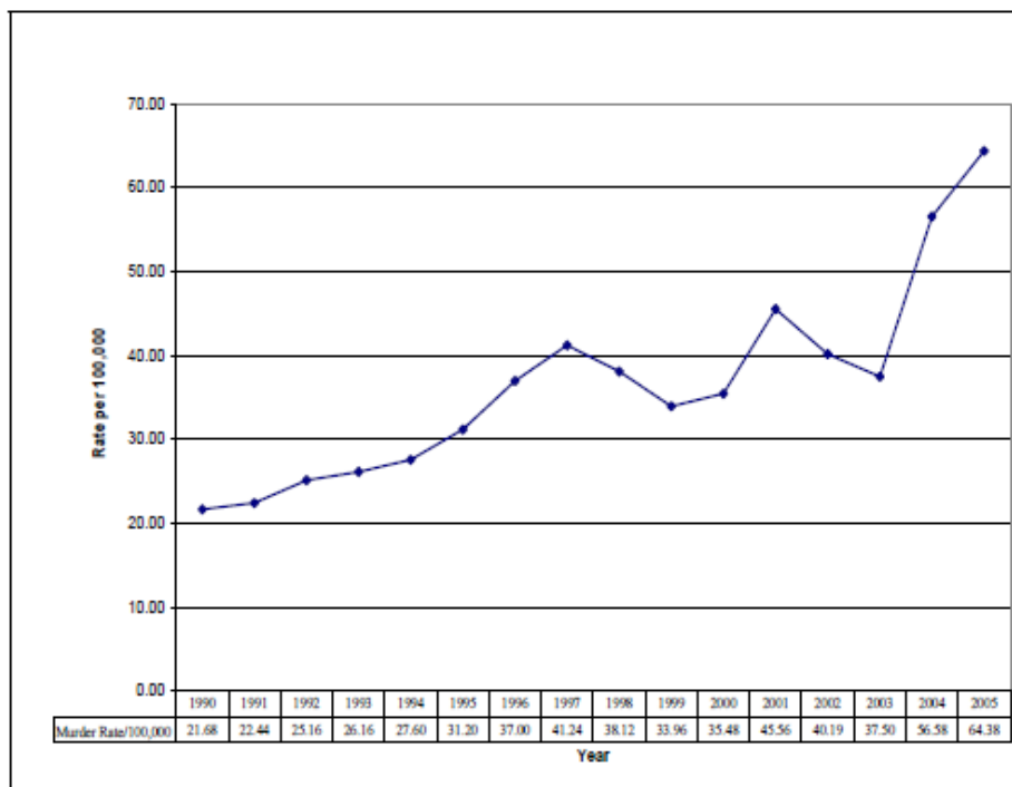
Figuur 2. Jamaica's Murder Rate per 100,000: 1990 – 2005.
