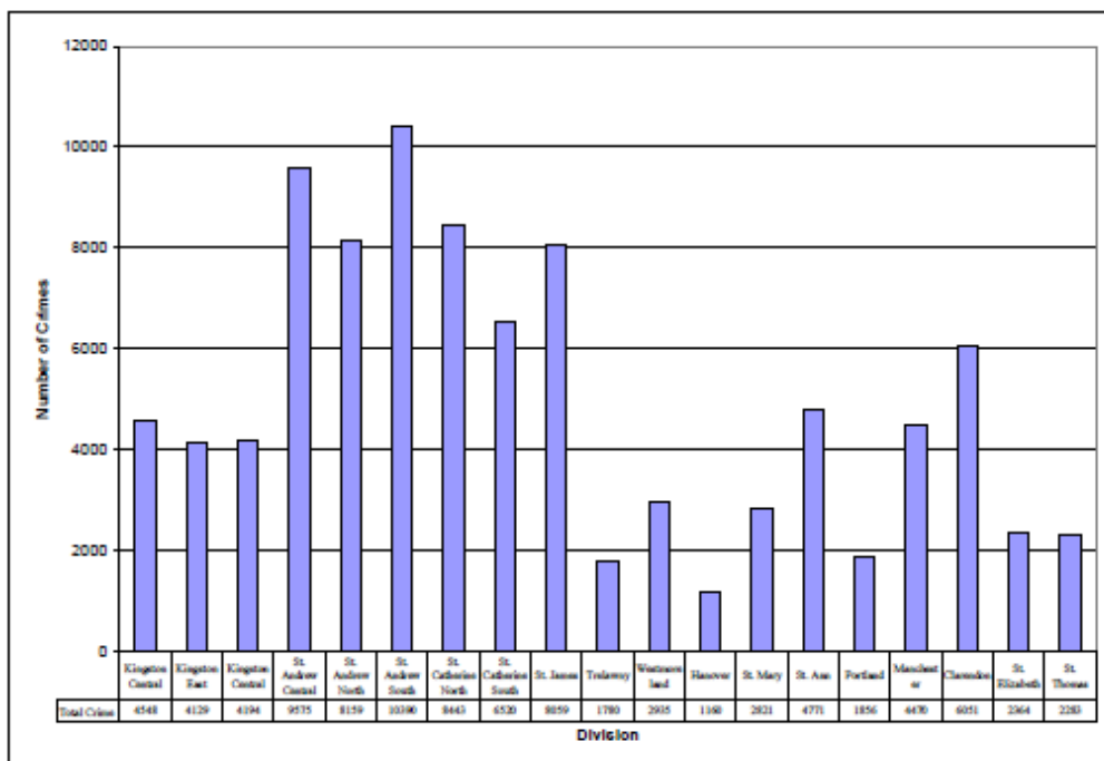
Figuur 4. Total Crime by Police Divisions: 1996 – 2005.
