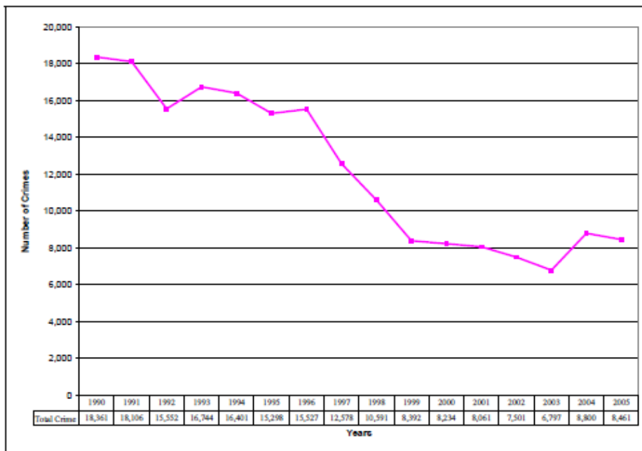
Figuur 3. Total Crime for Jamaica: 1990 – 2005.
